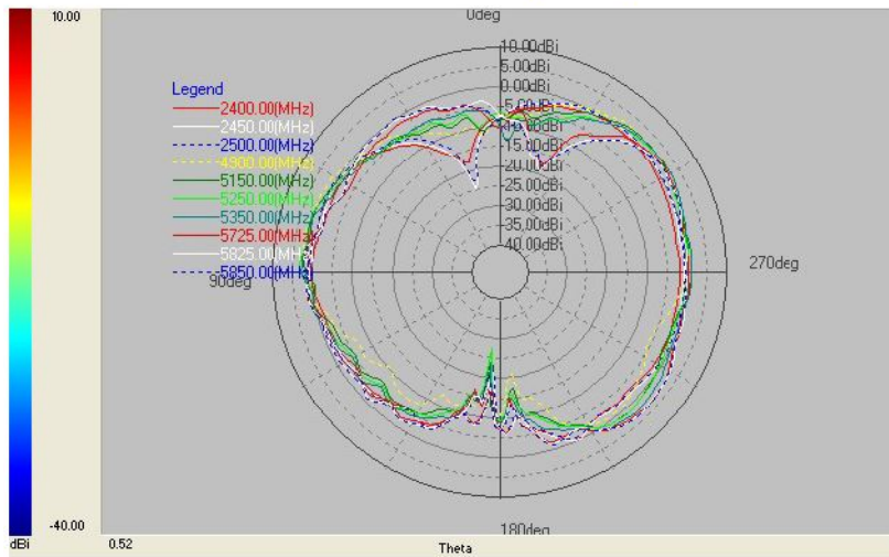
Y-Z Plane (E-total)
