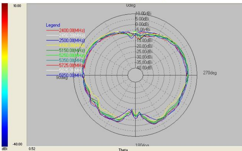
X-Z Plane (E-total)
