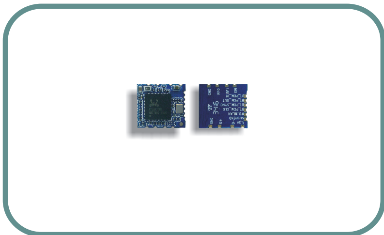
802.11 b/g/n with Bluetooth 4.0 Combo 1T1R, SMT Type, USB Module
